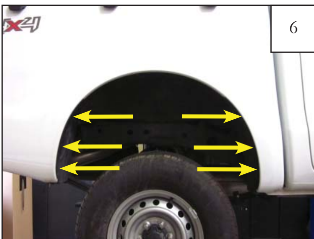
Using a #2 Phillips Screwdriver and or pry tool remove 6 pieces of factory hardware from the rear wheel well and discard. Note: Some vehicle models will have factory mudflaps. These will need to be removed for proper installation of flares.
